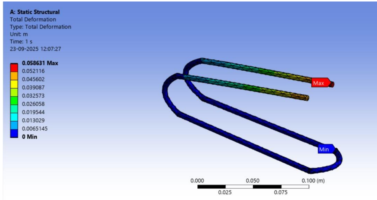
FIGURE 1 Model (A4) > Static Structural (A5) > Solution (A6) > Total Deformation > Total Deformation
