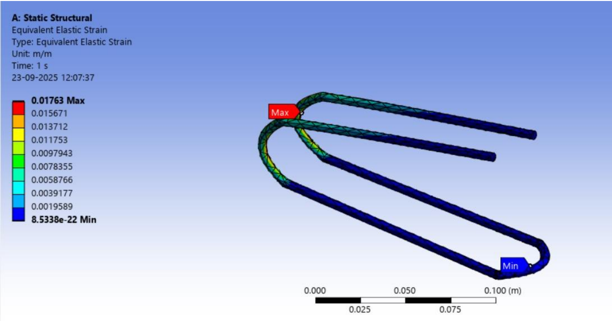
FIGURE 9 Model (A4) > Static Structural (A5) > Solution (A6) > Equivalent Elastic Strain > Equivalent strain
